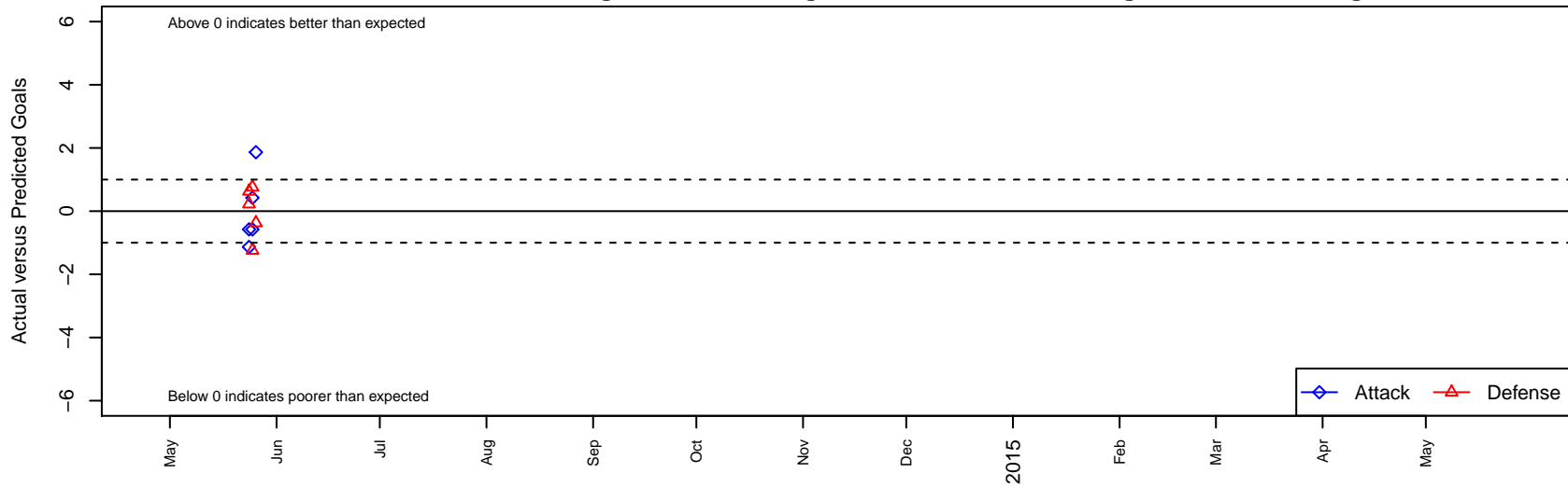
Aguilas United –Unk B96 Dots are actual minus expected GF (blue circles) and GA (red triangles). Blue line is smoothed change in attack strength. Red is smoothed change in defense strength.
